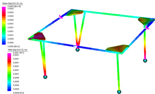
Deflection under worst load
