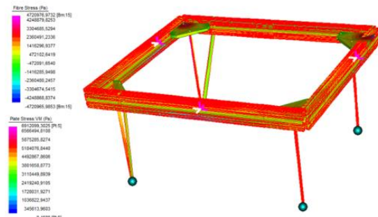
Vin Mises stress under load
